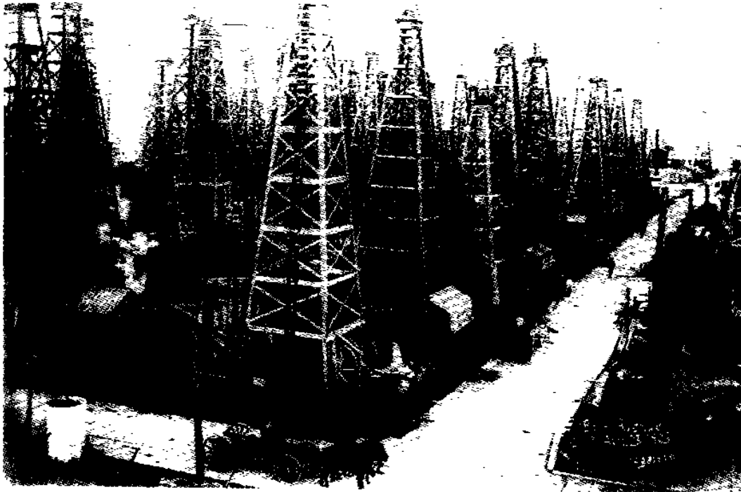
Figure 4 1903. Horses and carts travel down the plank road called Boiler Avenue which provided access to Spindletop's boiler locations. Wells were drilled so close together that a man could walk from one rig floor to another without ever touching the ground. Every well was a gusher. Reproduced with permission from Ohio University Press and Knowles.
